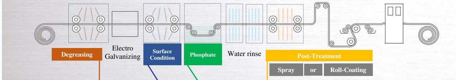
Process chart example of EGL ( Electro Galvanizing Line)
